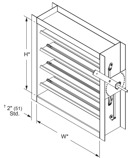
Model AC-82 *Damper dimensions furnished approximately net I.D..
