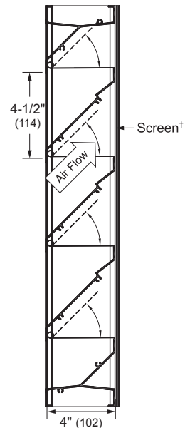
Vertical Section
