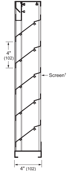
Vertical Section
