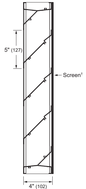
Vertical Section
