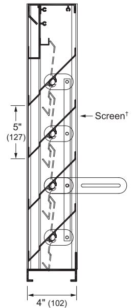
Vertical Section
