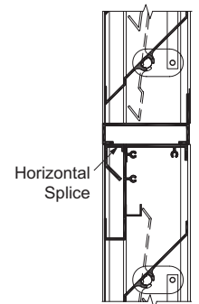
Horizontal Mullion (standard)
