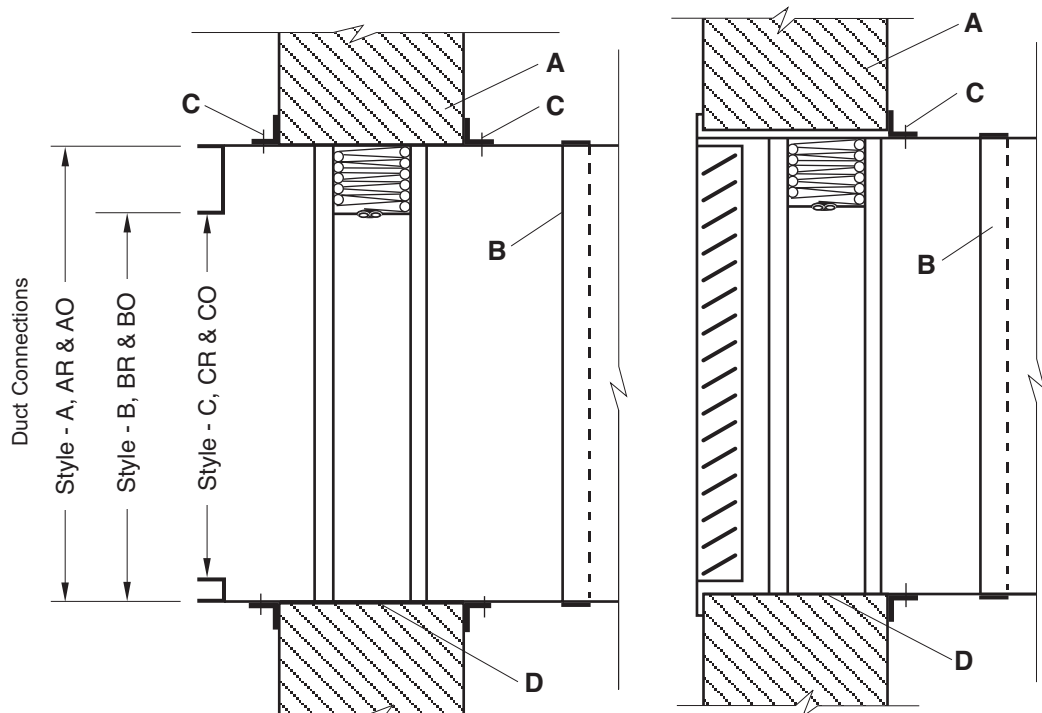
Damper Installation For Typical Fire Rated Partition
