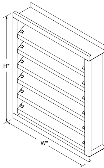
Model SJ-430 (standard)
